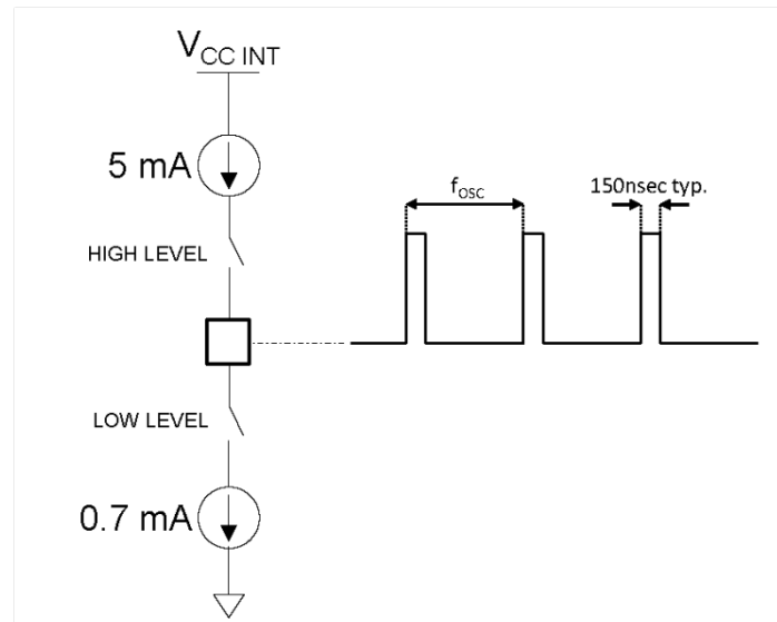
Figure 49. L6986H synchronization driving capability
