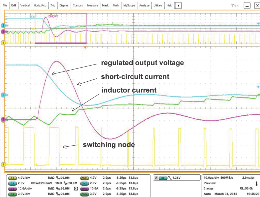
Figure 32. Zoomed waveforms
