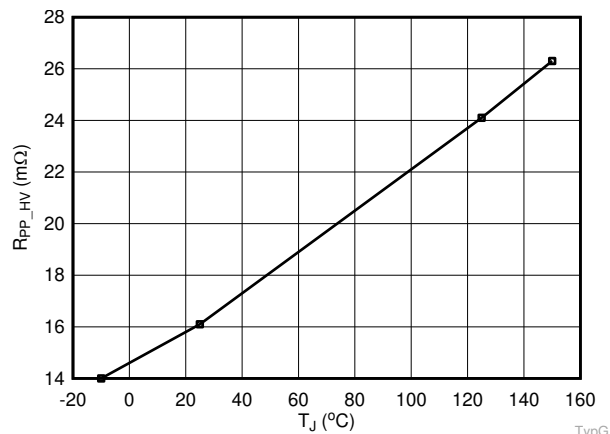
Figure 7-5. R_{PPHV} vs. Temperature for TPS25750D
