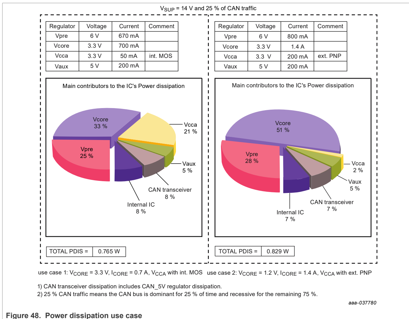
Figure 48. Power dissipation use case
