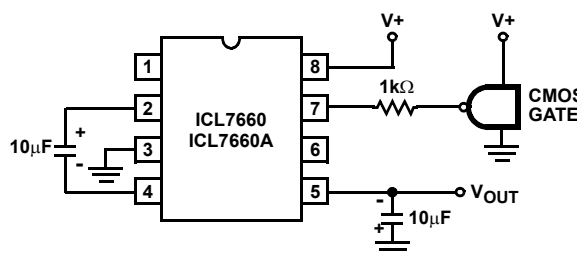
FIGURE 17. EXTERNAL CLOCKING
