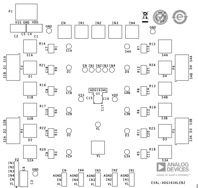
Figure 3. EVAL-ADG1634LEBZ Silkscreen
