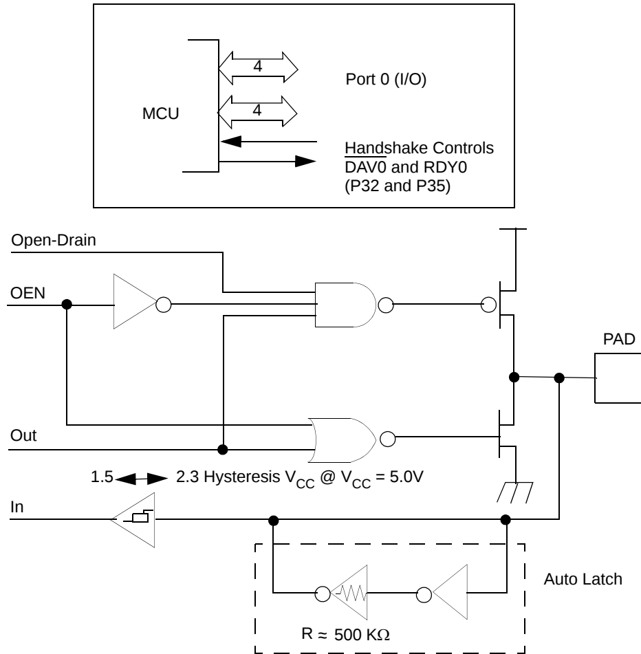
Figure 18. Port 0 Configuration
