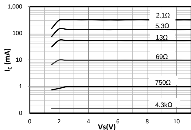
Figure 5. I_C vs. V_S (Parameter R_{EXT}=(\Omega) )
