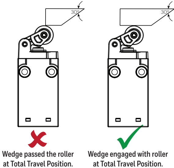
Figure 17. Wedge Actuation
