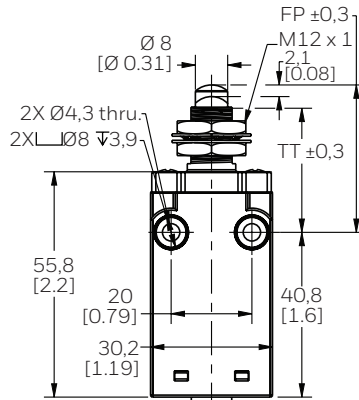
Figure 12. Panel-Mount Pin Plunger N Dimensions
