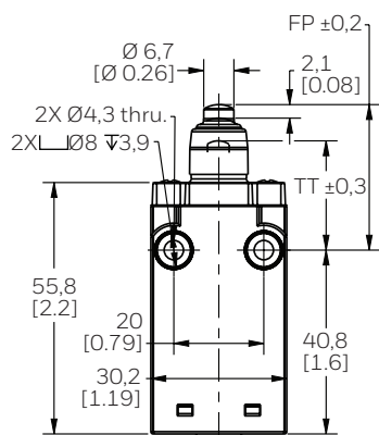
Figure 11. Pin Plunger with Boot Seal M Dimensions
