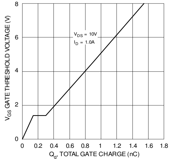
Fig. 10 Gate Charge
