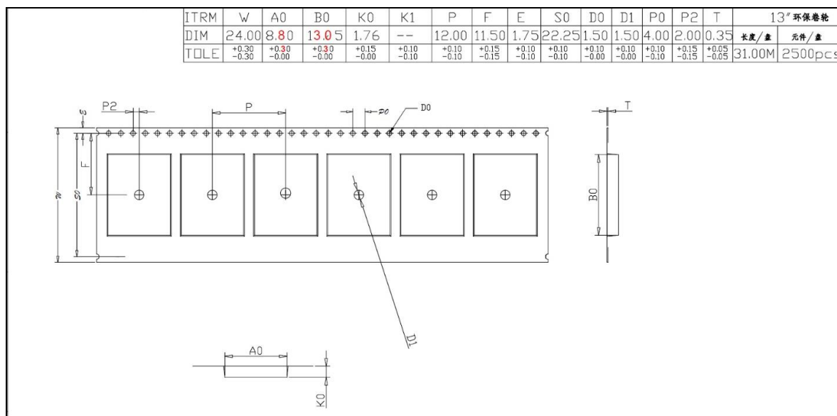
Figure 18: Tape specifications
