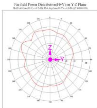
Figure 12: Antenna patterns
