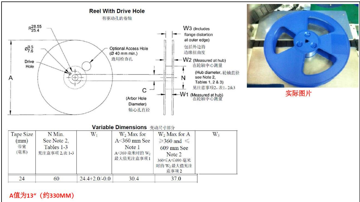
Figure 17: Reel specifications
