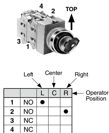
Contact Block Mounting Position and Contact Arrangement Chart
