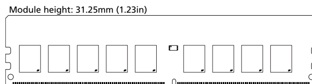
Figure 1: 288-Pin UDIMM (MO-309, R/C-E1)
