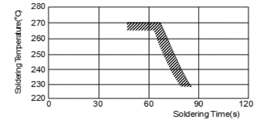
[ Allowable Reflow Soldering Temperature and Time ]
