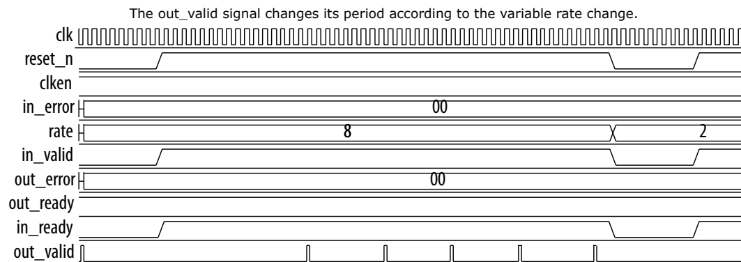
Figure 7. Variable Rate Change Decimation CIC Filter Timing Diagram
