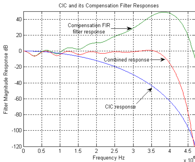
Figure 11. CIC and Compensation Filter Responses
