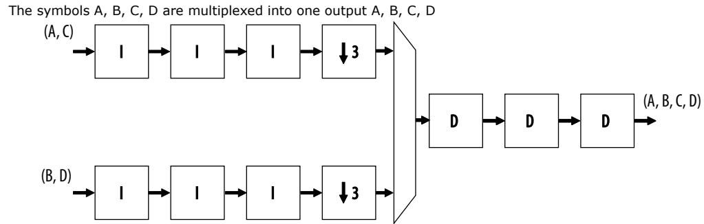
Figure 8. Multiple Input Single Output Architecture For Four Channels
