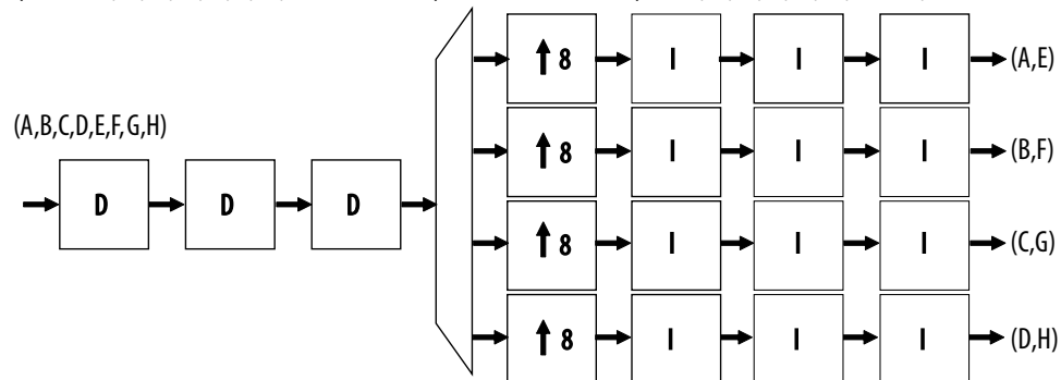
Figure 9. Single Input Multiple Output Architecture with Eight Channels
