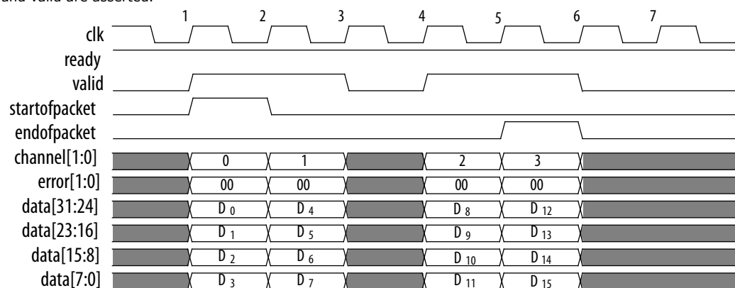
Figure 13. Packet Data Transfer
