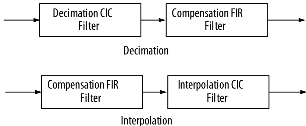
Figure 10. Using a CIC Compensation FIR Filter
