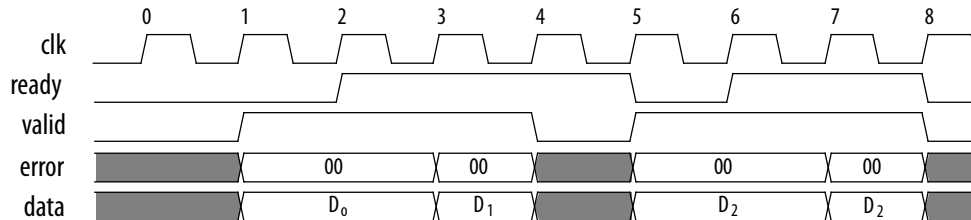
Figure 12. Avalon Streaming Interface Timing with READY_LATENCY=0
