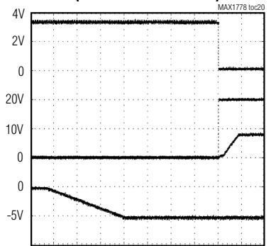
POWER-UP SEQUENCE (CIRCUIT OF FIGURE 10)
