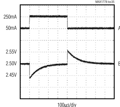
EXTERNAL LINEAR-REGULATOR LOAD-TRANSIENT RESPONSE
