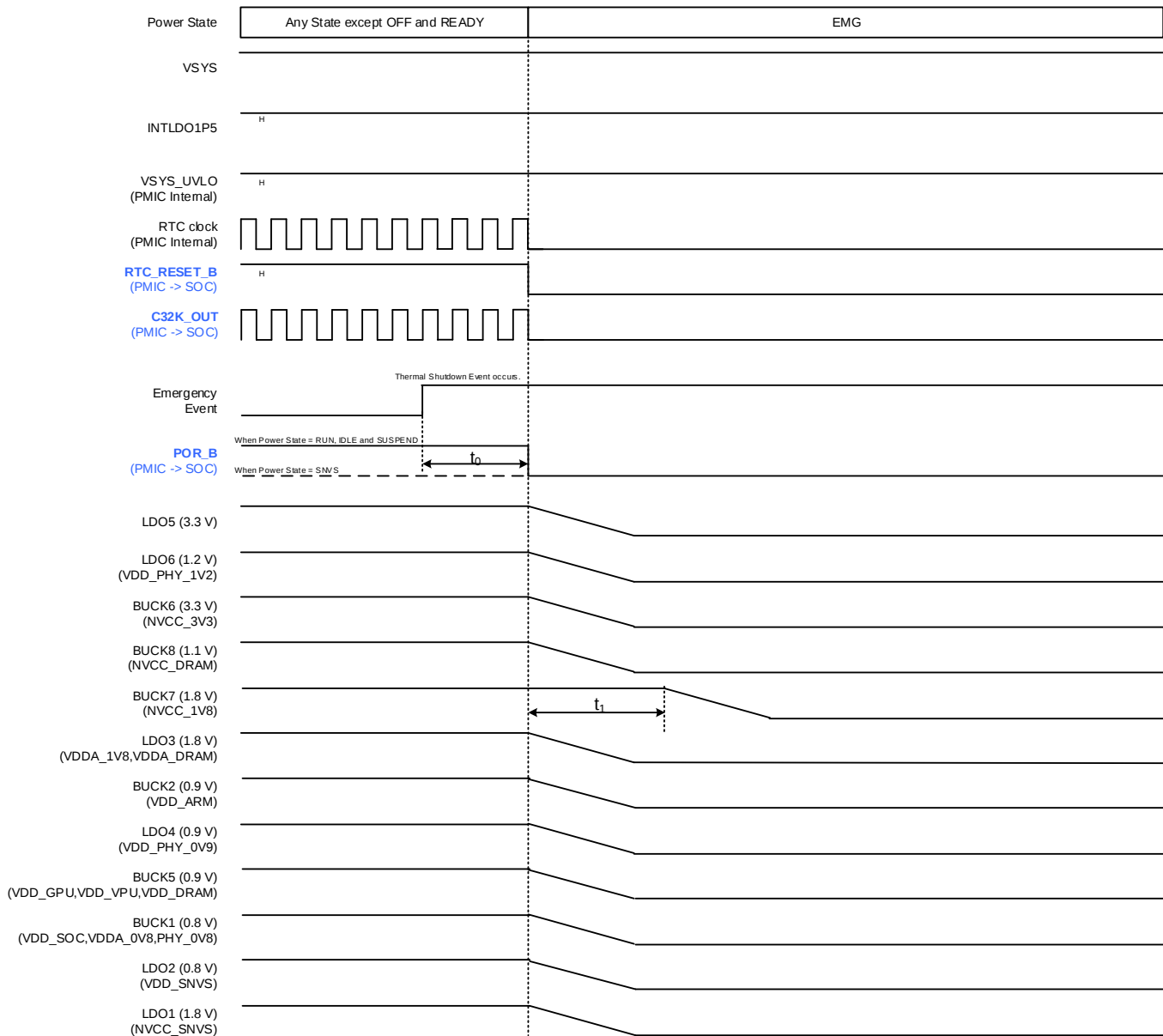
Figure 3-29. Emergency Shutdown
