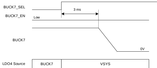
Figure 5-12. LDO4 Voltage Source Switching
