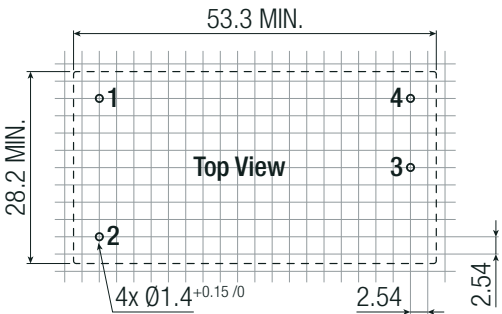
Recommended Footprint Detail
