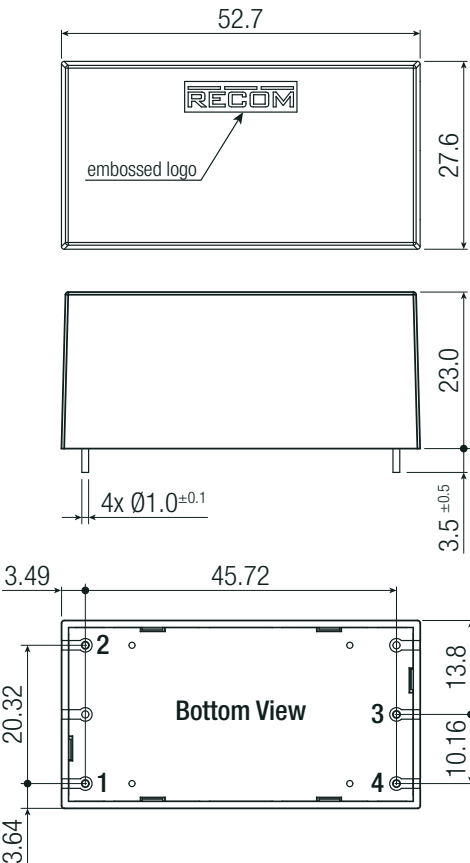
Dimension Drawing THT printmount version (mm)
