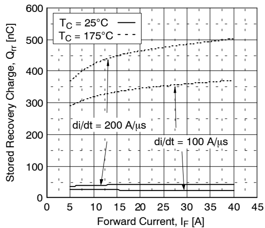
Figure 23. Stored Charge
