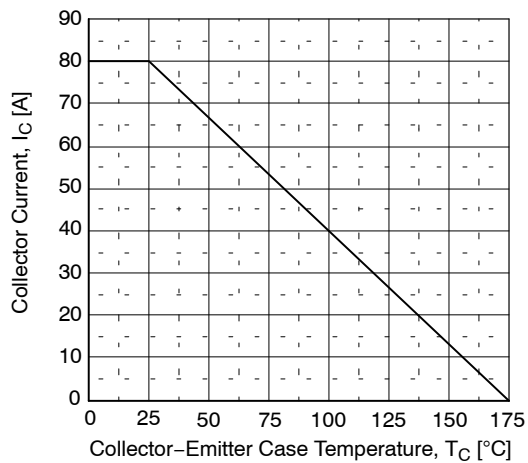
Figure 19. Current Derating
