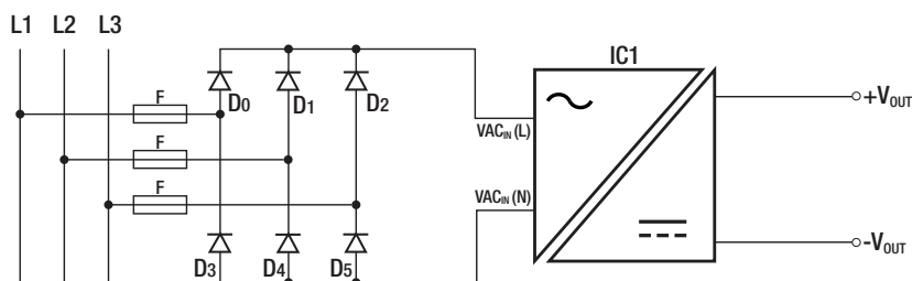
Phase Redundancy B6U Application
