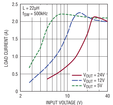
Maximum Load Current vs V IN , PWM Mode
