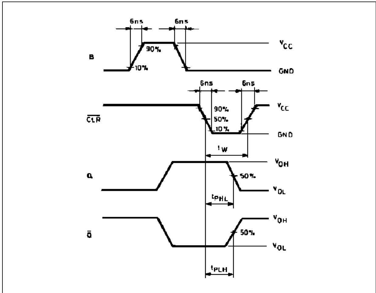
WAVEFORM 2 : MINIMUM PULSE WIDTH ( \overline{\text{CLR}} ), PROPAGATION DELAY TIME ( f=1\text{MHz} ; 50% duty cycle)
