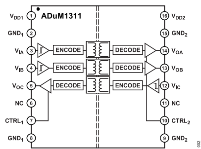
Figure 2. ADuM1311
