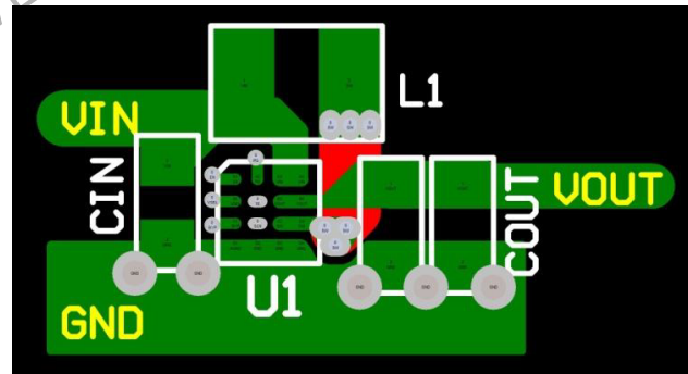
Figure 29. Layout Recommendation
