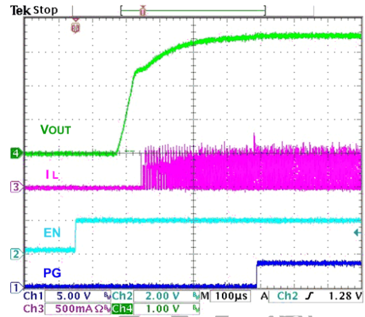
Figure 18. Startup, 50 \Omega Load, V_{IN} = 2.5\text{ V} , V_{OUT} = 3.5\text{ V}
