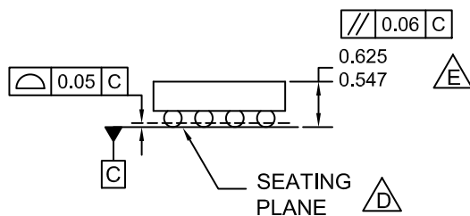
SIDE VIEWS
