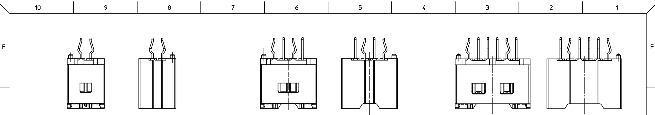
2~3 極形状 (ロック面及び反ロック面) 4~5 極形状 (ロック面及び反ロック面) 6~7 極形状 (ロック面及び反ロック面) FIGURE OF 2-3 CIRCUIT (LOOK SIDE AND UN-LOCK SIDE) FIGURE OF 4-5 CIRCUIT (LOOK SIDE AND UN-LOCK SIDE) FIGURE OF 6-7 CIRCUIT (LOOK SIDE AND UN-LOCK SIDE)
