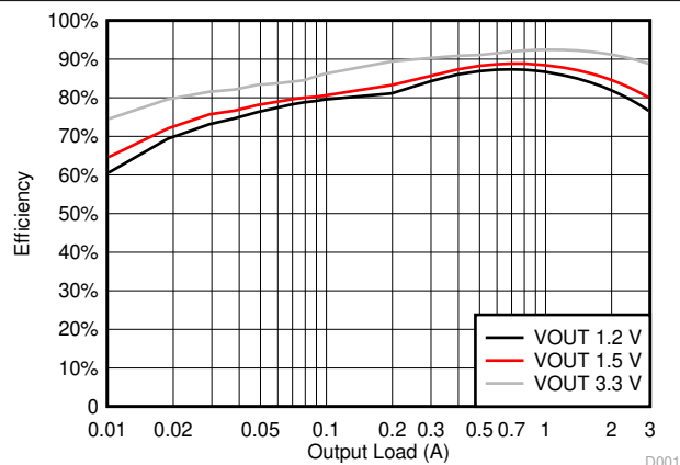
Figure 6-1. BUCK1 Efficiency
