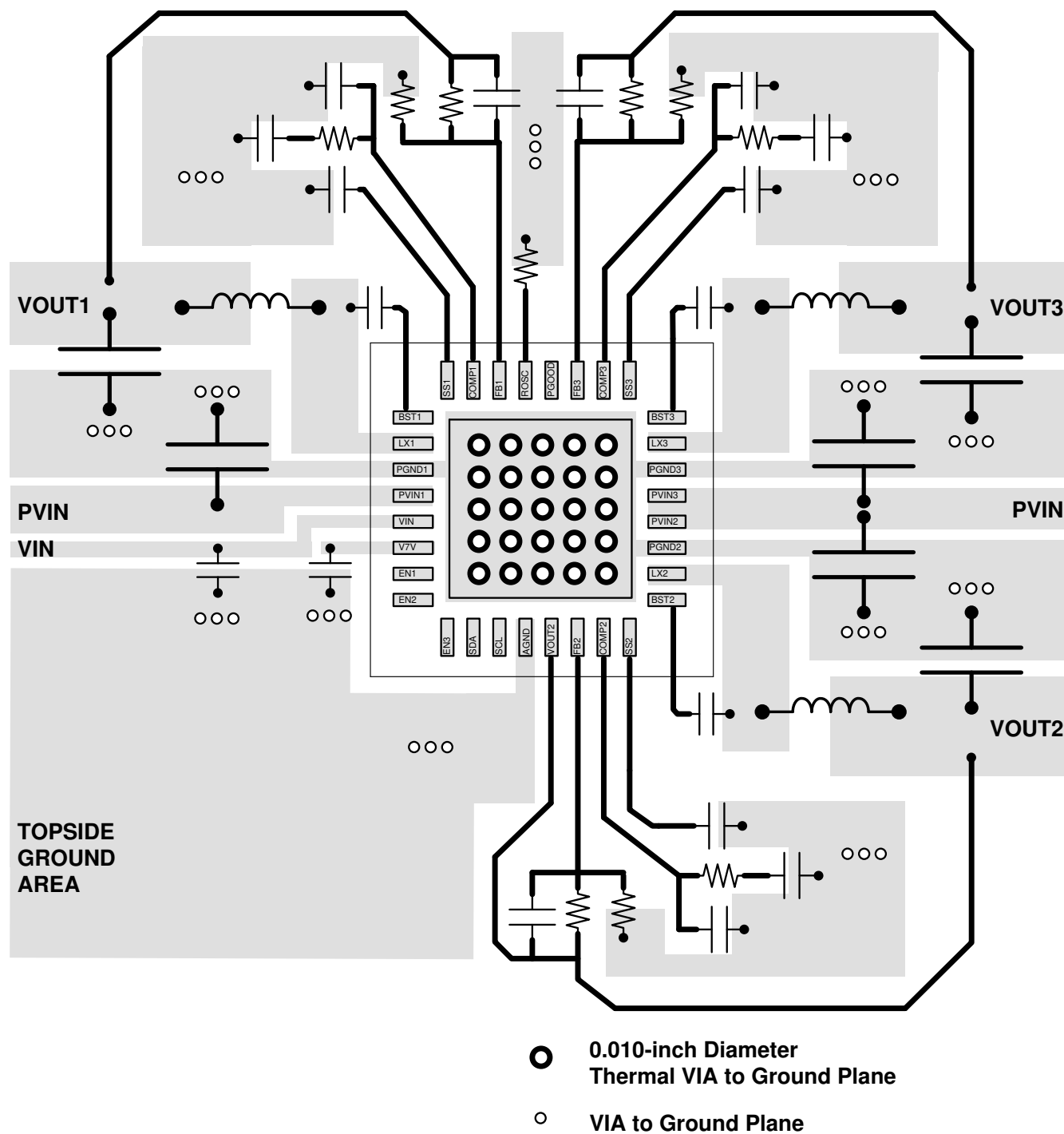
Figure 8-25. PCB Layout
