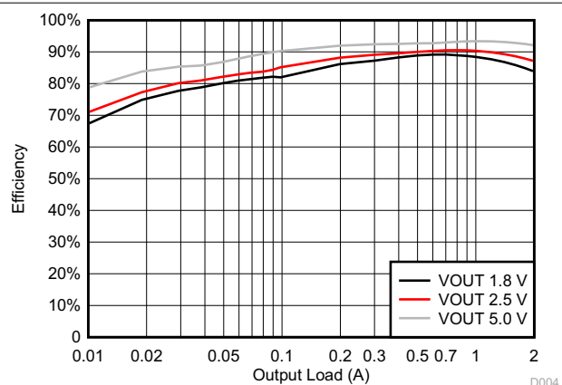
Figure 6-3. BUCK3 Efficiency
