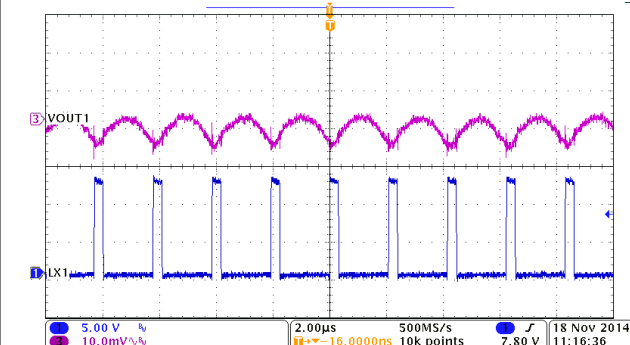
Figure 8-6. BUCK1, Output Voltage Ripple
