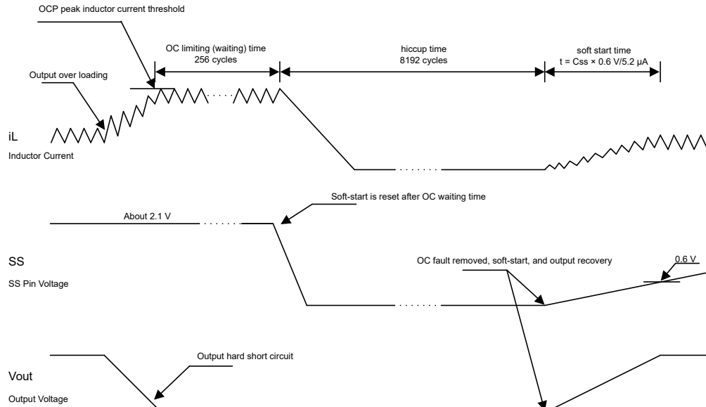
Figure 7-11. Overcurrent Protection
