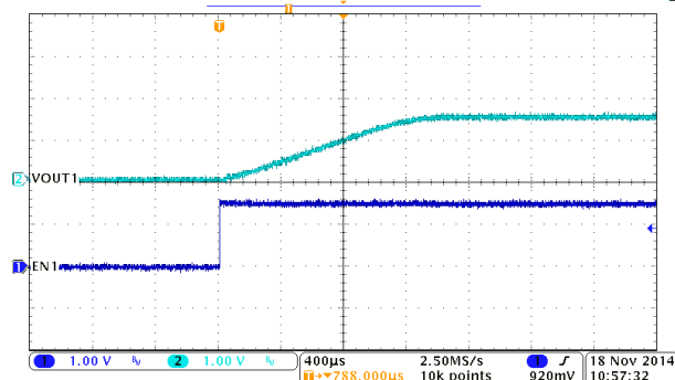
Figure 8-3. BUCK1, Soft Start
