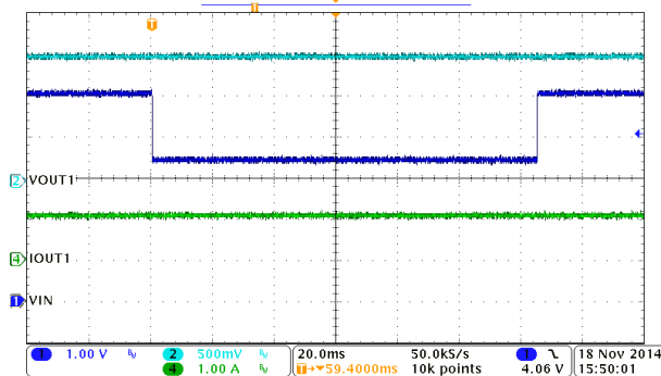
Figure 8-23. Operation at VIN Drop to 2.5 V
