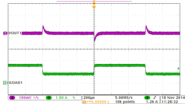
Figure 8-9. BUCK1, Load Transient
