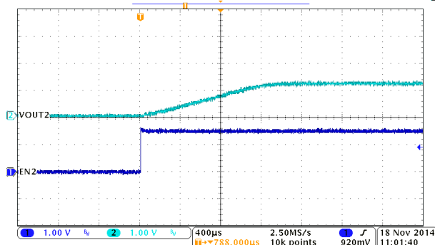
Figure 8-4. BUCK2, Soft Start
