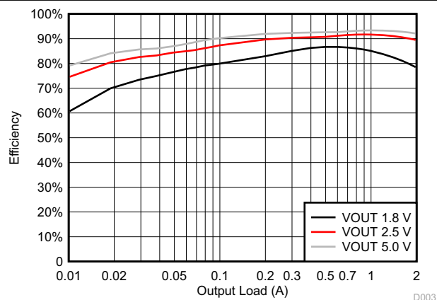
Figure 6-2. BUCK2 Efficiency
