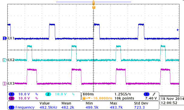
Figure 8-21. 180° Out-of-Phase
