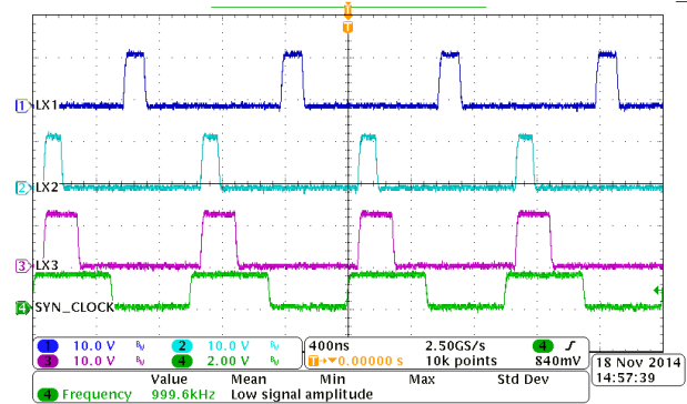
Figure 8-22. Synchronization with External Clock
