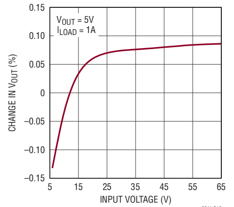
Line Regulation
