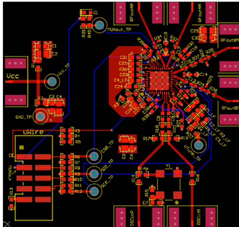
Figure 8-13. Recommended Layout
