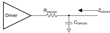
Figure 8-9. ZDRIVER Circuit
