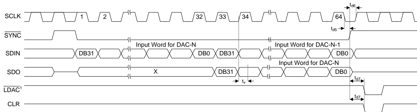
Figure 2. Daisy-Chain Timing
