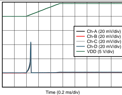
DAC unloaded
