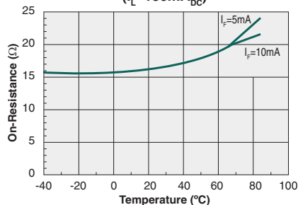
Typical On-Resistance vs. Temperature AC/DC Configuration ( I_L=150\text{mA}_{\text{DC}} )
