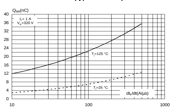
Figure 6: Reverse recovery charges versus di_F / dt (typical values)
