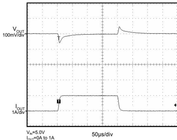
Transient Response ( V_{OUT} = 1.5V ; 0A to 1A)
