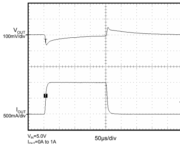
Transient Response ( V_{OUT} = 3.3V ; 0A to 1A)
