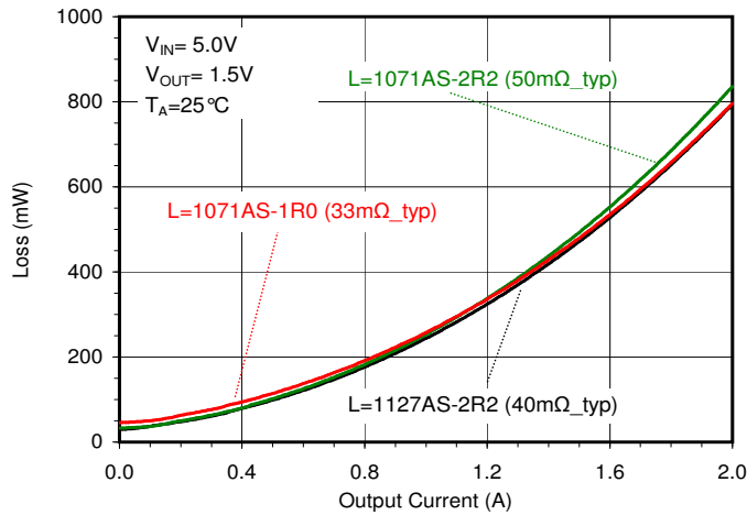
Total Loss vs. Load Current ( V_{OUT}=1.5V )
