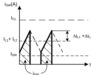
Figure 16. Switch Current Waveform in a Cuk Converter.
