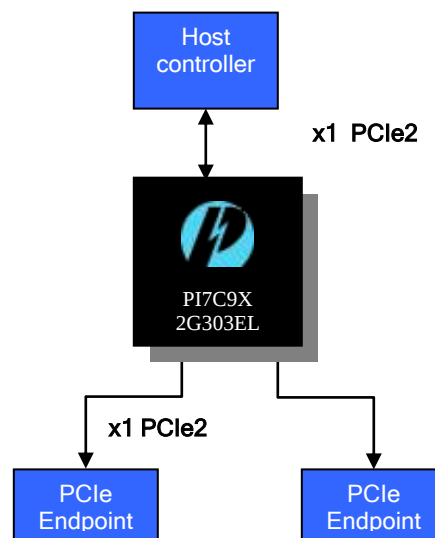
PI7C9X2G303EL – Application Example
