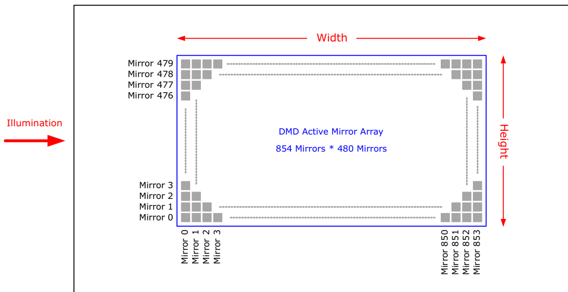
Figure 15. Micromirror Array Physical Characteristics
