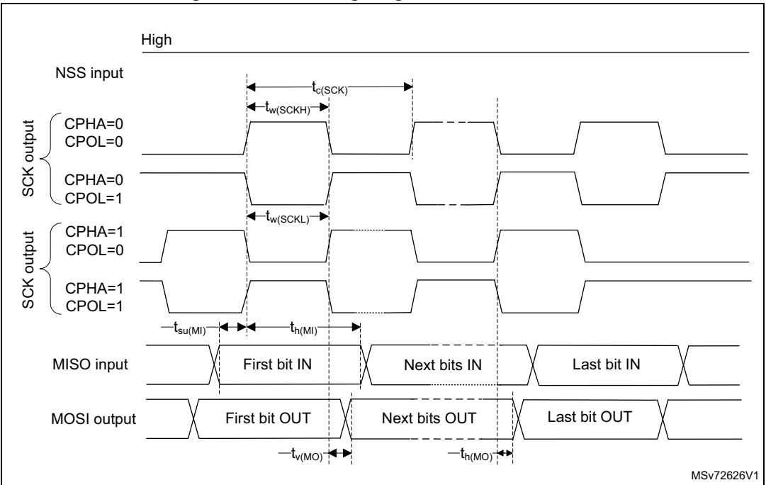
Figure 42. SPI timing diagram - master mode (1)
