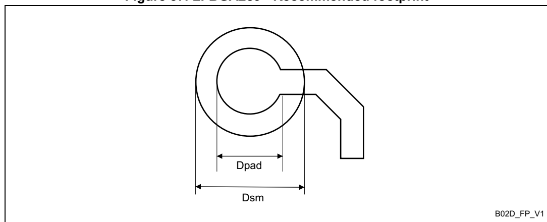
Figure 57. LFBGA289 - Recommended footprint
