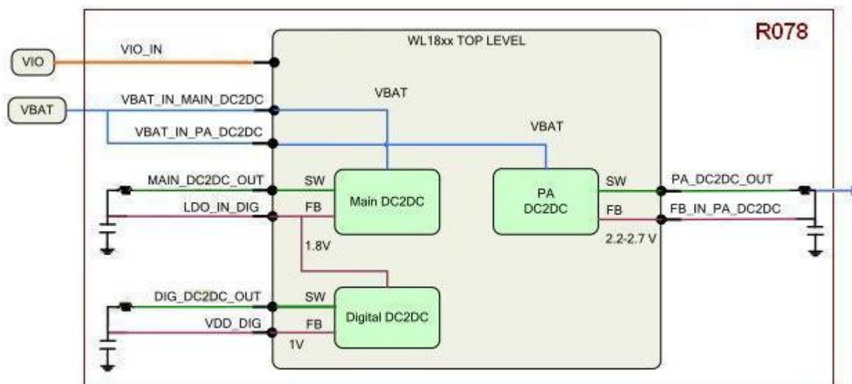
Figure 3-3 Internal DC2DC's
