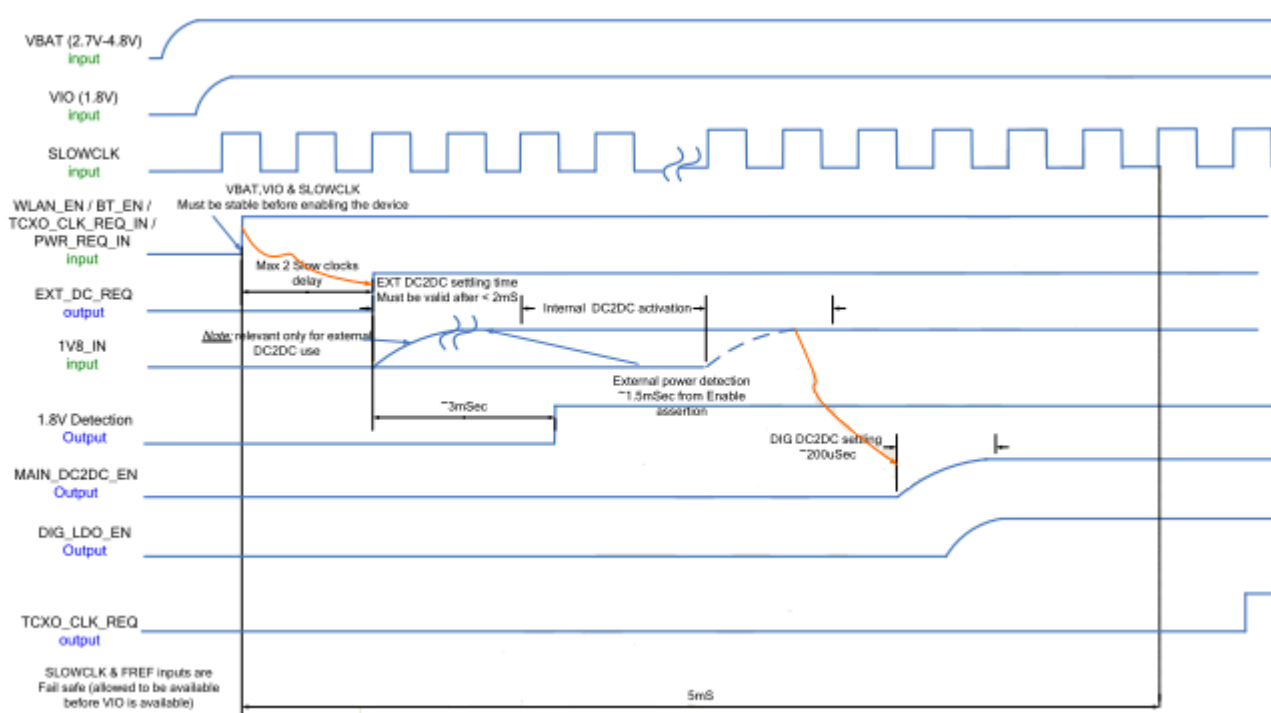
Figure 3-4 Chip Top-level Power Up Sequence
