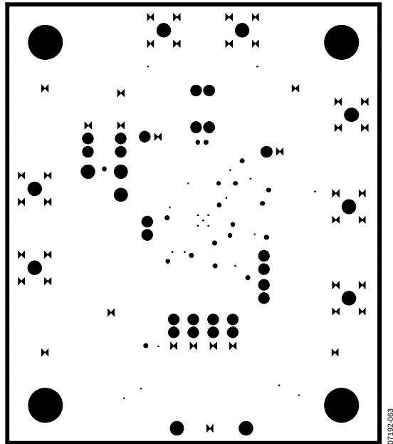
Figure 75. AD8260-EVALZ Ground Plane
