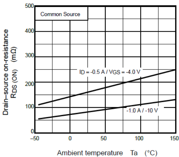
Fig. 7.5 R_{DS(ON)} - T_a
