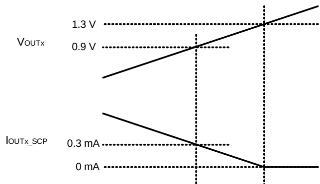
Figure 18. OUTx pin Short Circuit Current
