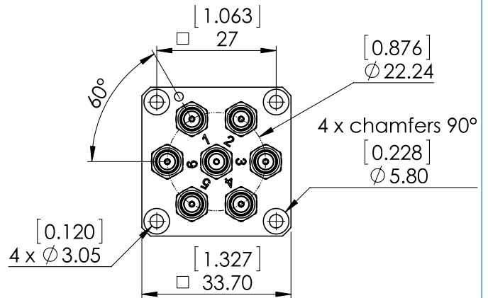
Micro-D model
