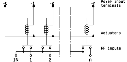
NORMALLY OPEN WITH POSITIVE COMMON R591 -0- -1-
