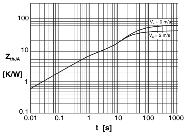
Fig. 4 Transient thermal resistance
