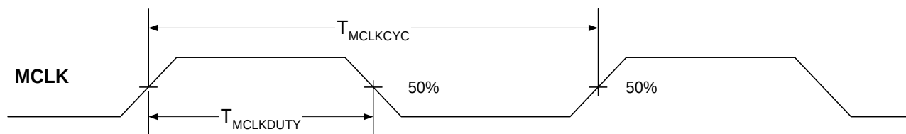
Figure 4.10. MCLK Timings
