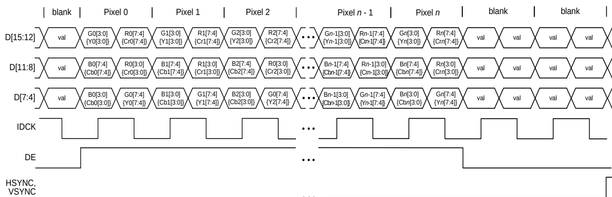
Figure 6.32. 12-Bit RGB/YCbCr 4:4:4 Separate Sync Timing (49-Ball Package)
