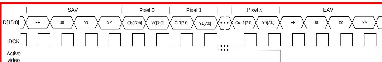
Figure 6.18. 8-Bit YC Mux 4:2:2 Embedded Sync Timing (81-Ball and 72-Pin Package)
