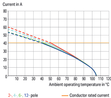
Current-carrying capacity curves PCB terminals blocks (2624-11xx) Pin spacing: 5 mm / Conductor cross-section: 6 mm 2 "f-st" Based on: EN 60512-5-2 / Reduction factor: 1
