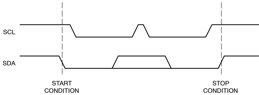
Figure 2. Start/Stop Timing
