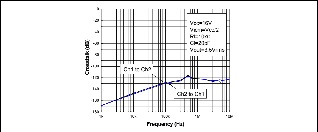
Figure 34. Crosstalk vs. frequency between operators on TSX9292 at V_{CC} = 16\text{ V}
