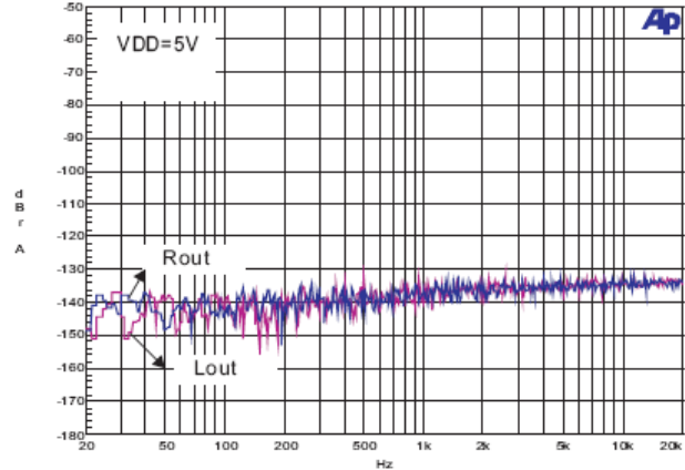
17. Noise Floor
