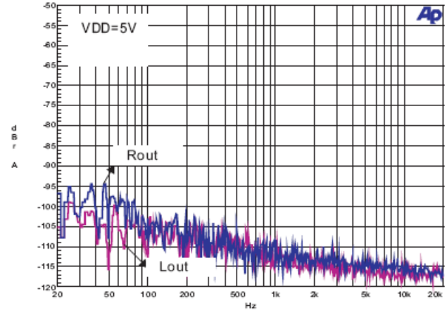
6. Noise Floor
