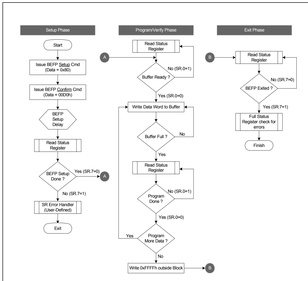
Figure 38: BEFP Flowchart
