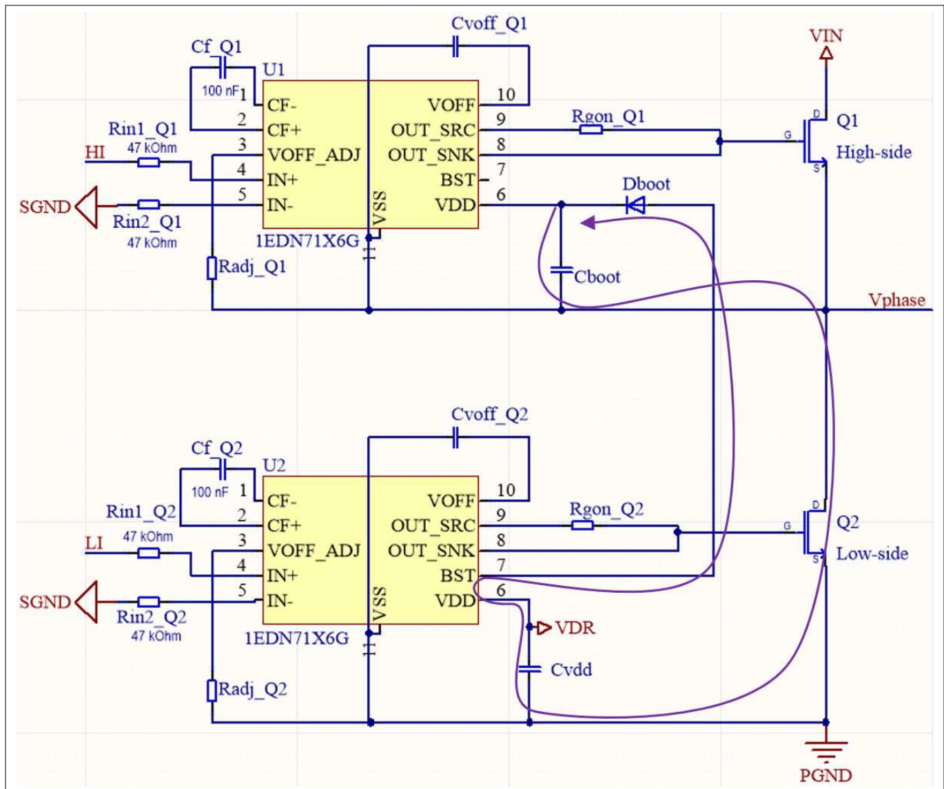
Figure 5 Half-bridge with active bootstrap clamping (CP enabled)
