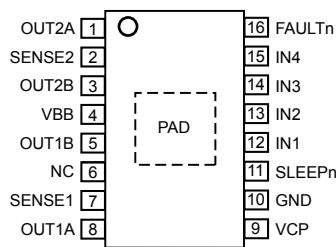
16-Lead TSSOP (LP) Package
