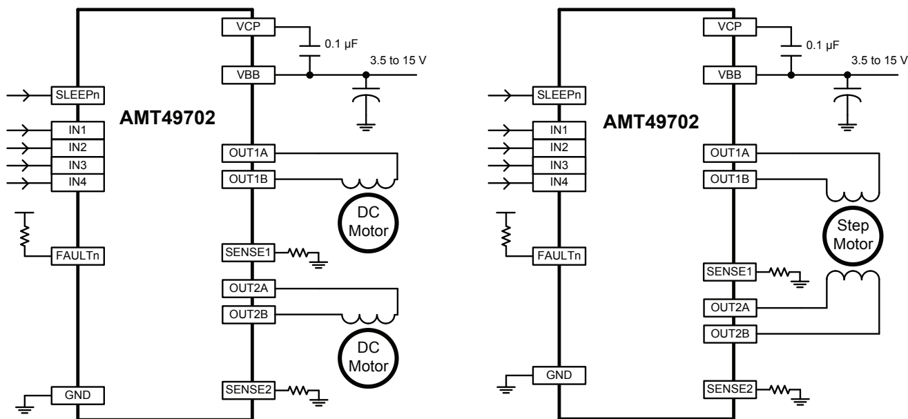
Figure 1: Typical Applications
